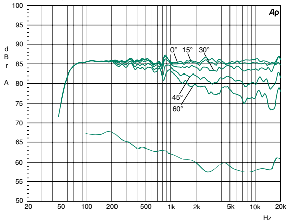
Genelec Oy 8330 horizontal off axis response level (dB) vs freq (Hz) 23 Sept 14
